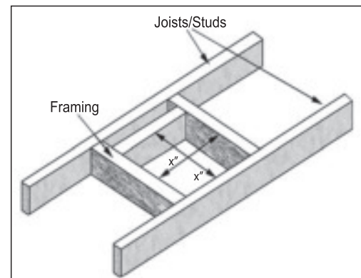
Figure 39: Vent Framing For Wall or Ceiling
