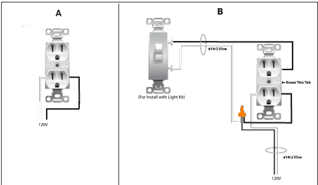
Figure 52: C60 Receptacle Wiring
