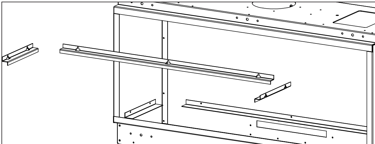
Figure 59: Panel I nstallation
