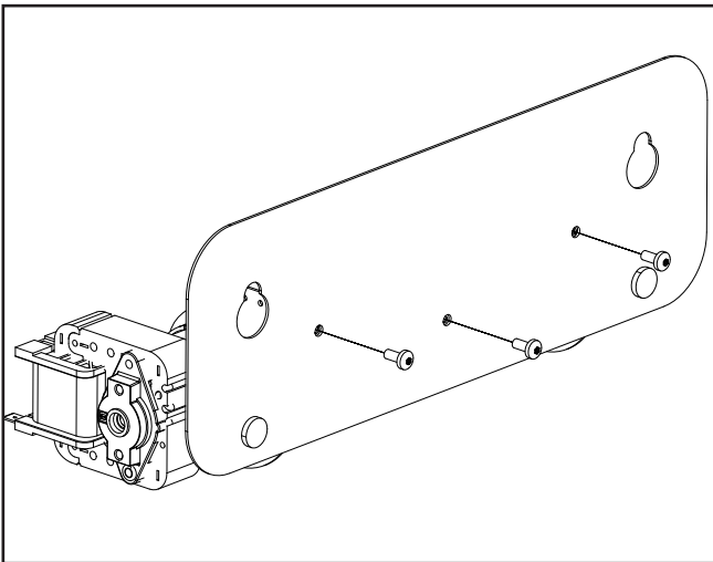
Figure 32: Fan Removal
