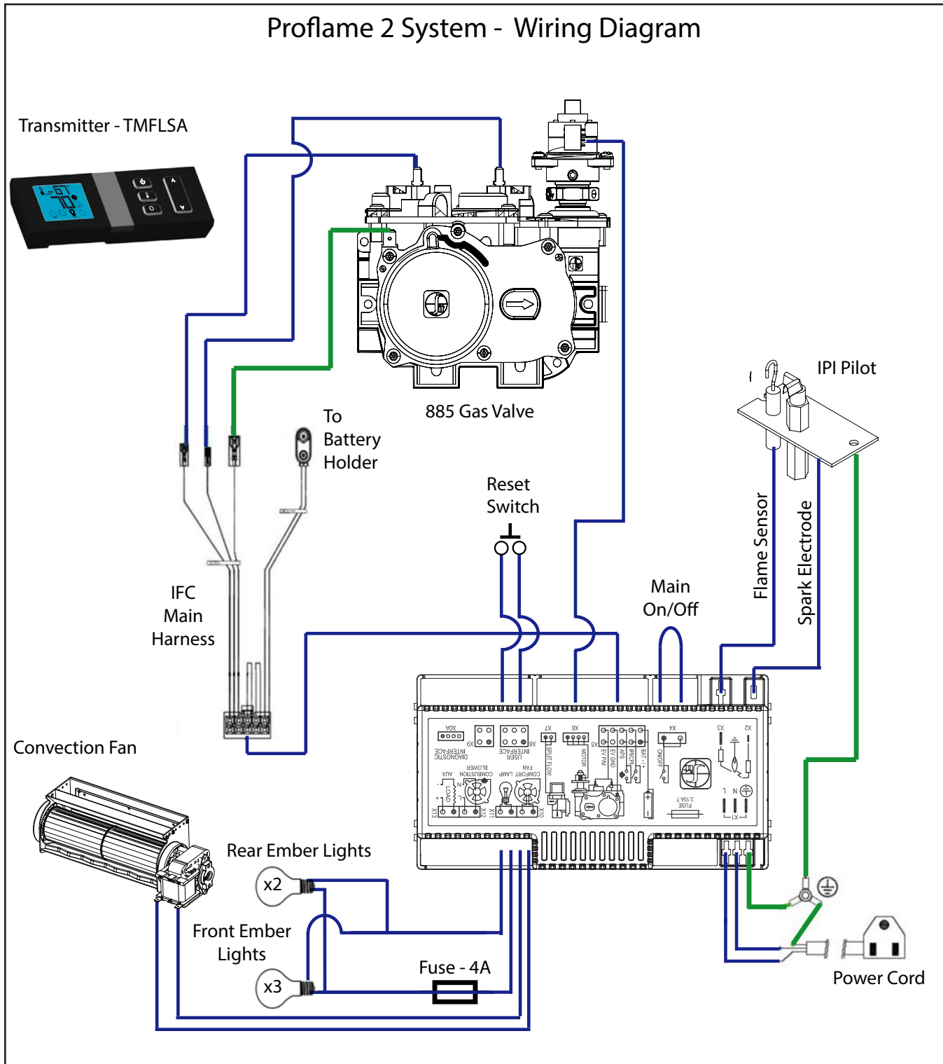
Figure 53: Wiring Schematic.
