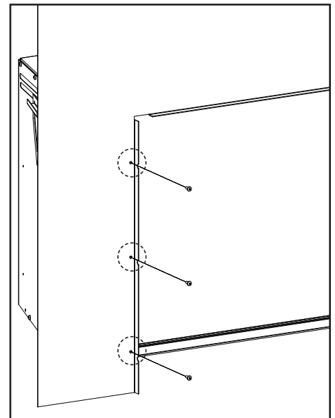
Figure 63: Screw Installation Locations.
