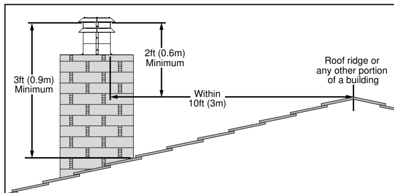
Figure 48: Roof Clearances.
